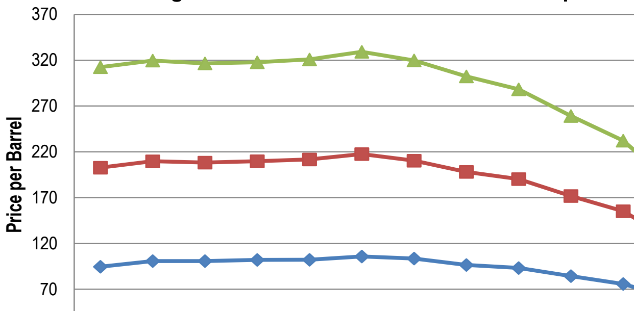
Fig 11: Trends for different world crude prices
