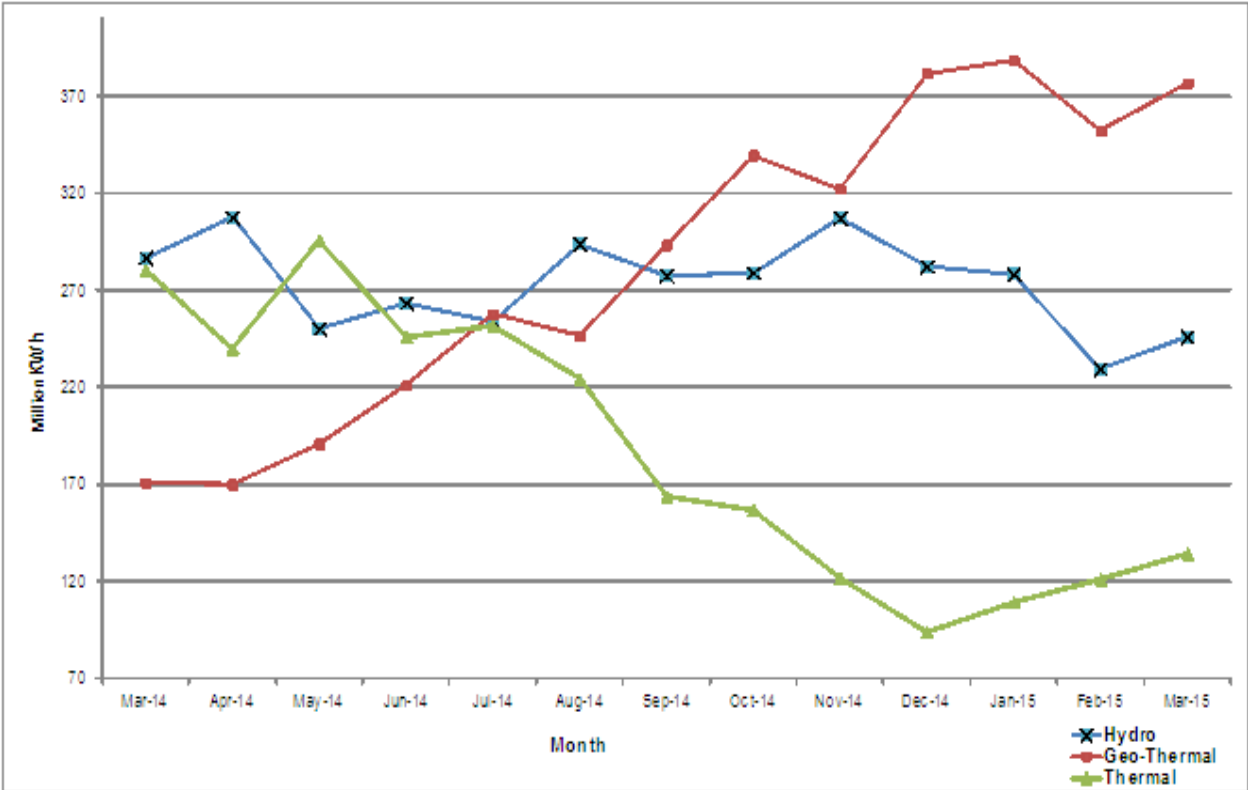
Fig.8: Electricity Generation by Source
