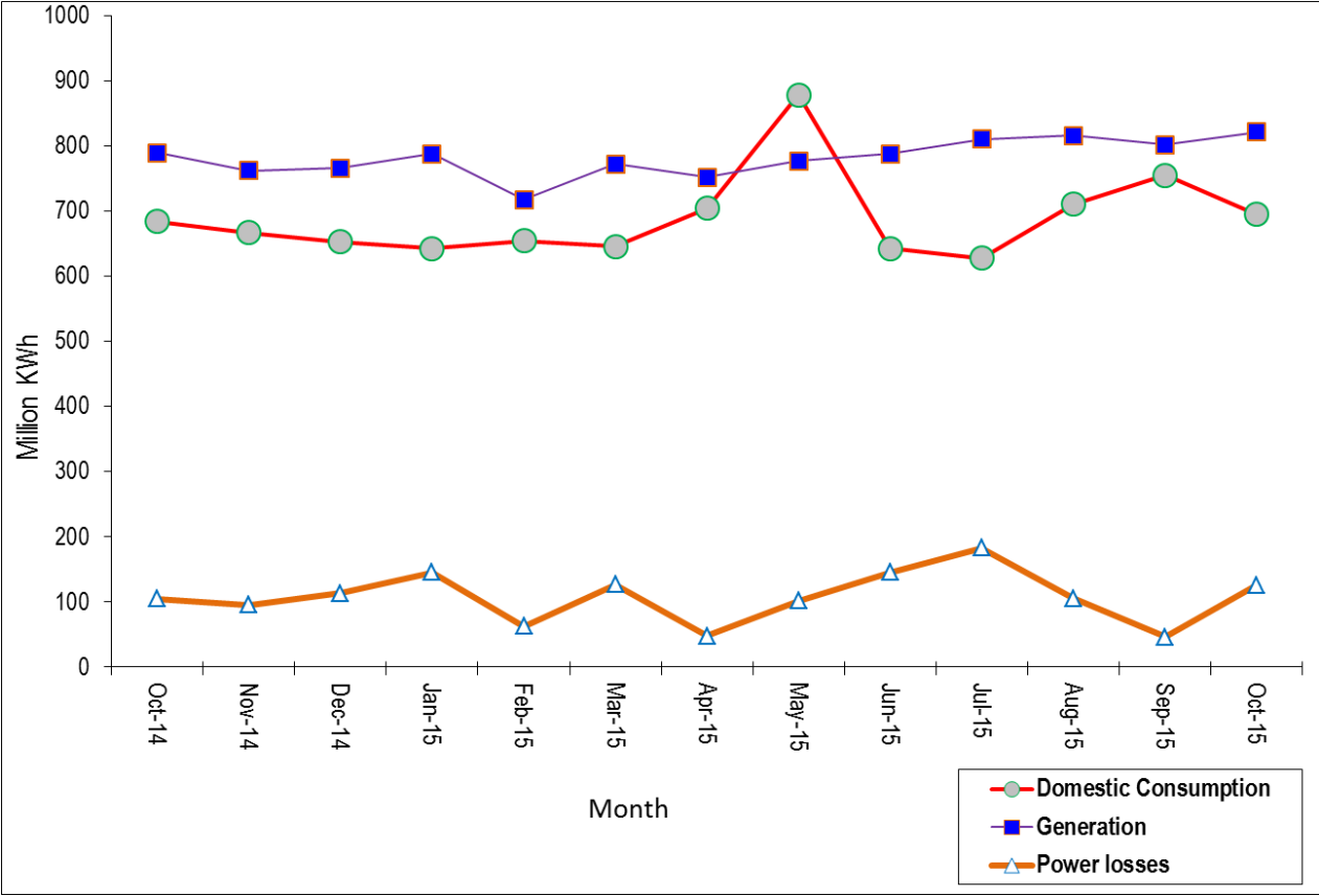
Fig.9: Electricity Generation, Consumption and Power Losses
