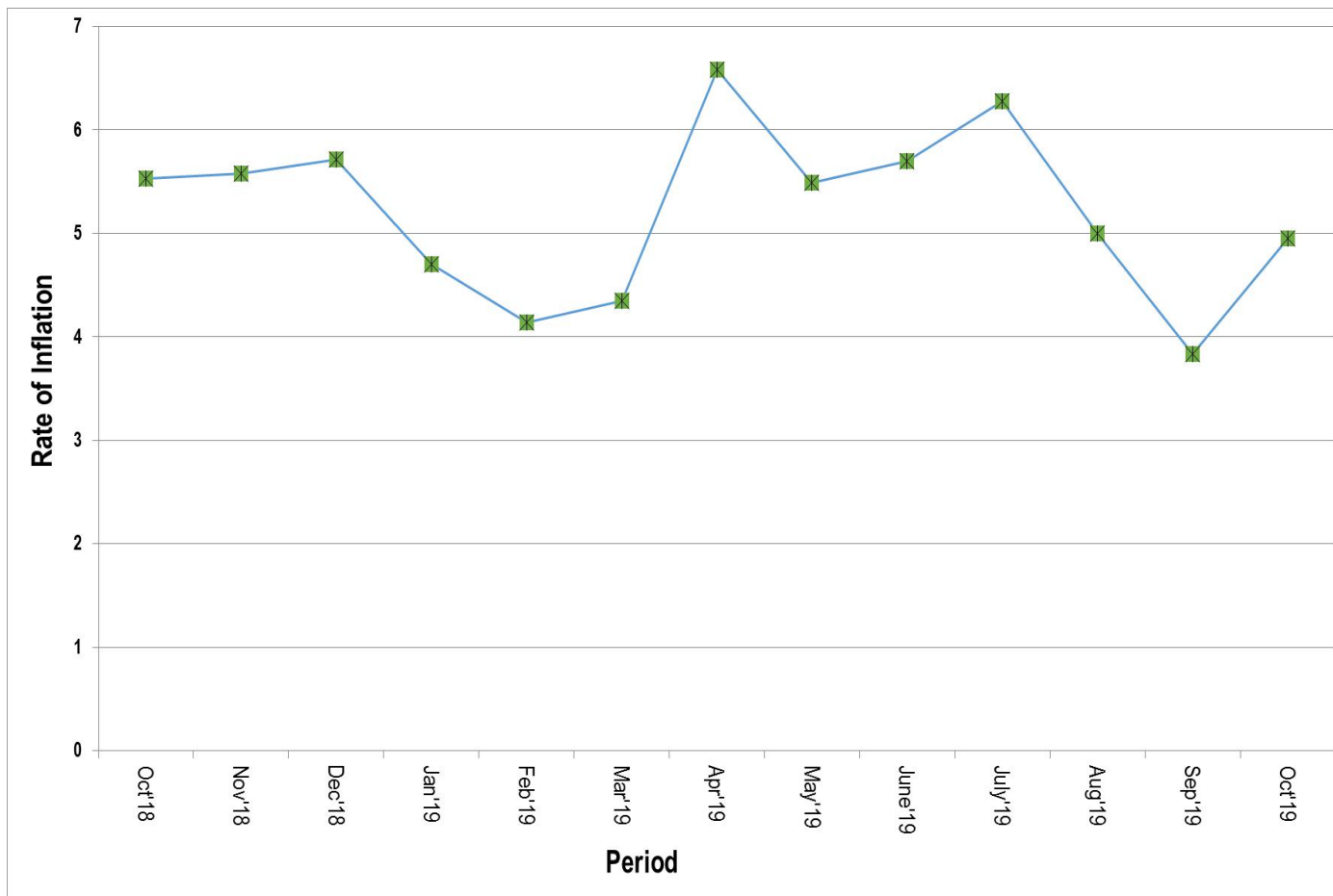
Fig. 1: Inflation rates
