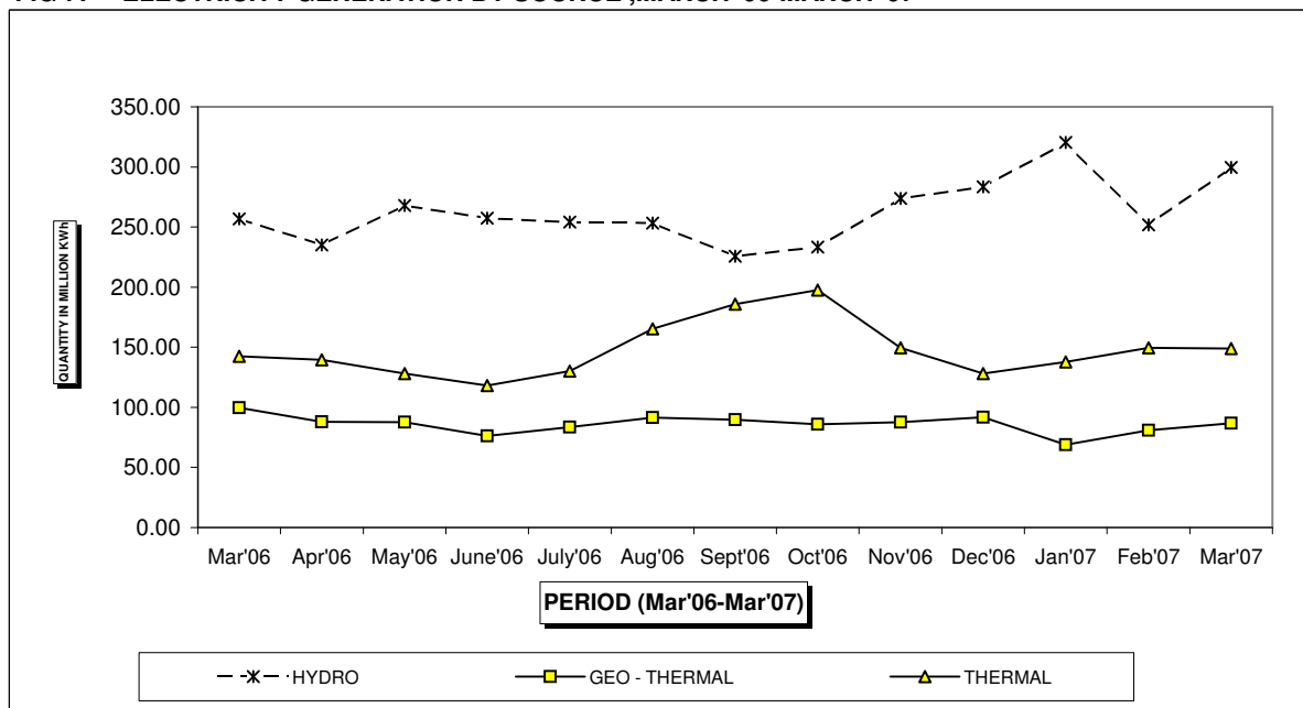
FIG 7: ELECTRICITY GENERATION BY SOURCE ,MARCH '06-MARCH '07
