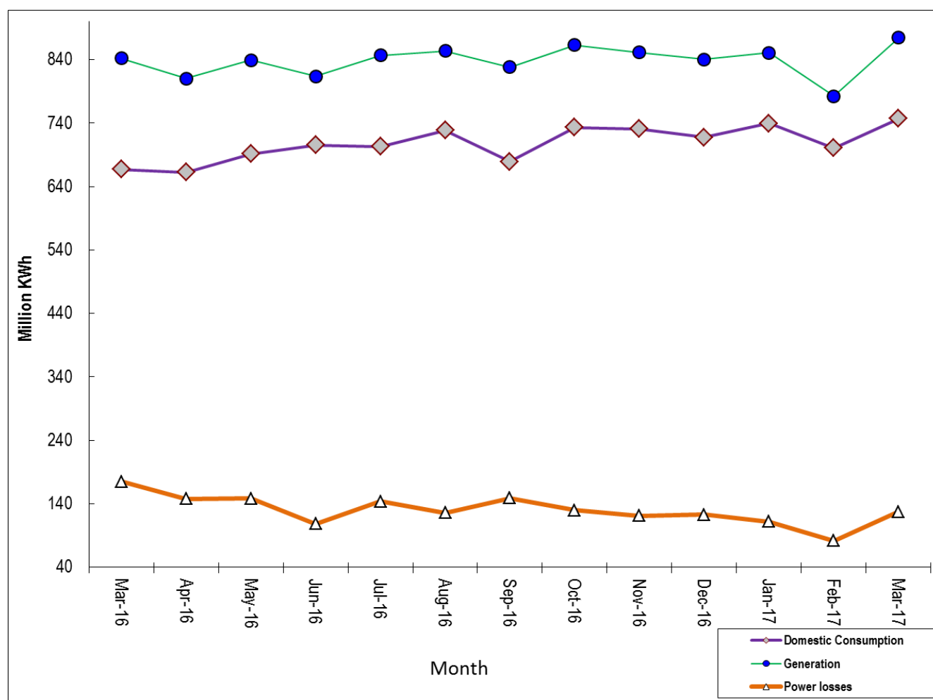
Fig. 9: Electricity Generation, Consumption and Power Losses
