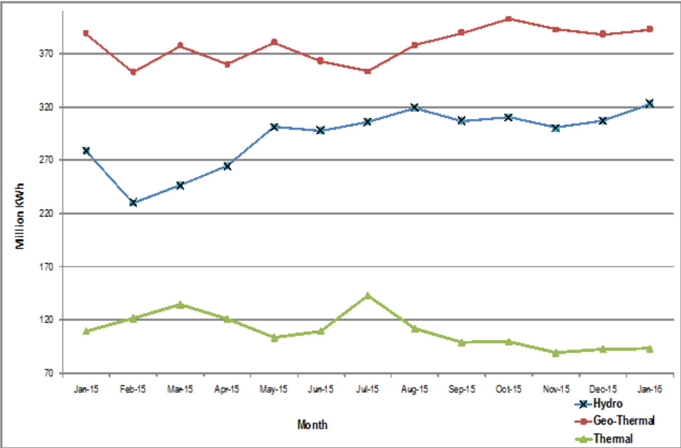
Fig.8: Electricity Generation by Source
