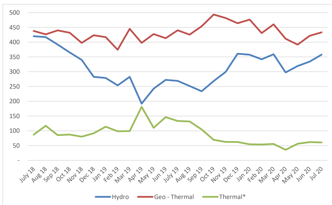
Fig. 7: Electricity Generation by Source
