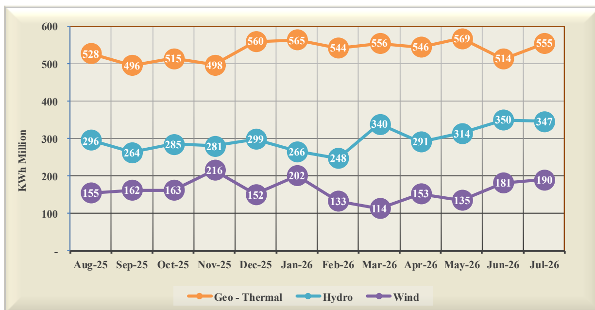
Figure 6: Electricity Generation by Source
