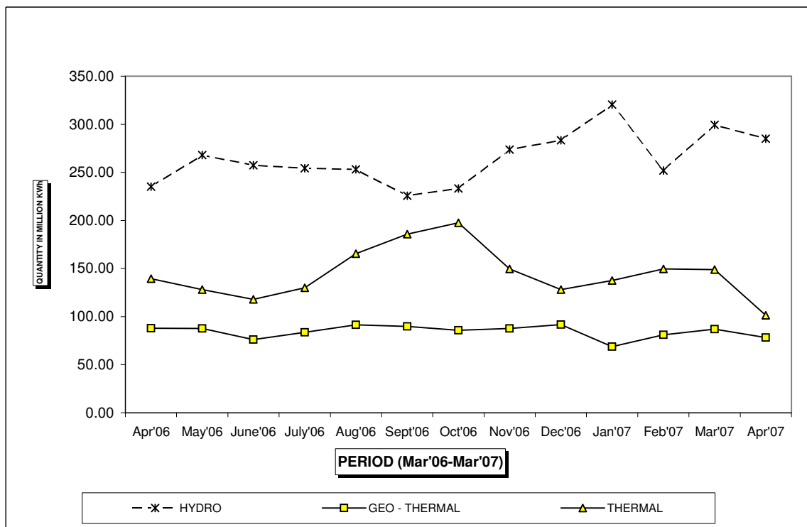
FIG 7: ELECTRICITY GENERATION BY SOURCE ,MARCH '06-MARCH '07
